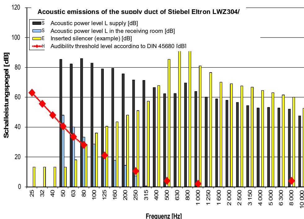
Figure 1: Acoustic emissions of supply duct of the unit Stiebel Eltron LWZ 504 [dB]
