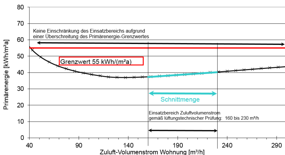
Figure 2: Application range of the unit Stiebel Eltron LWZ 304
